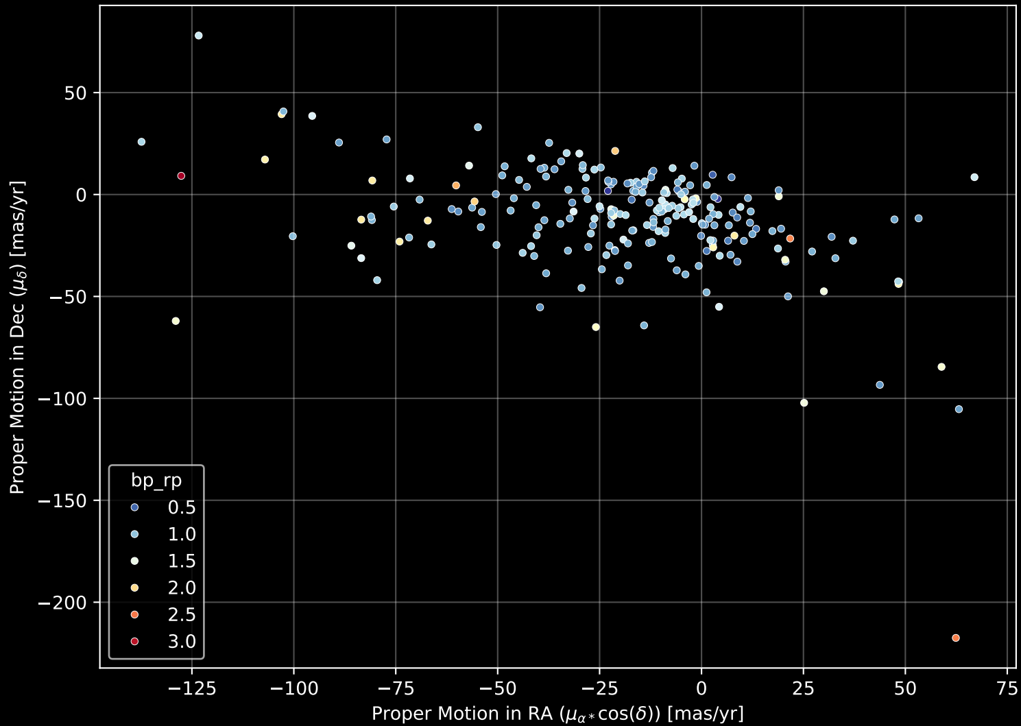
APOGEE DR17 Field: [040+88_MGA] Proper Motion Diagram (n= 231)
