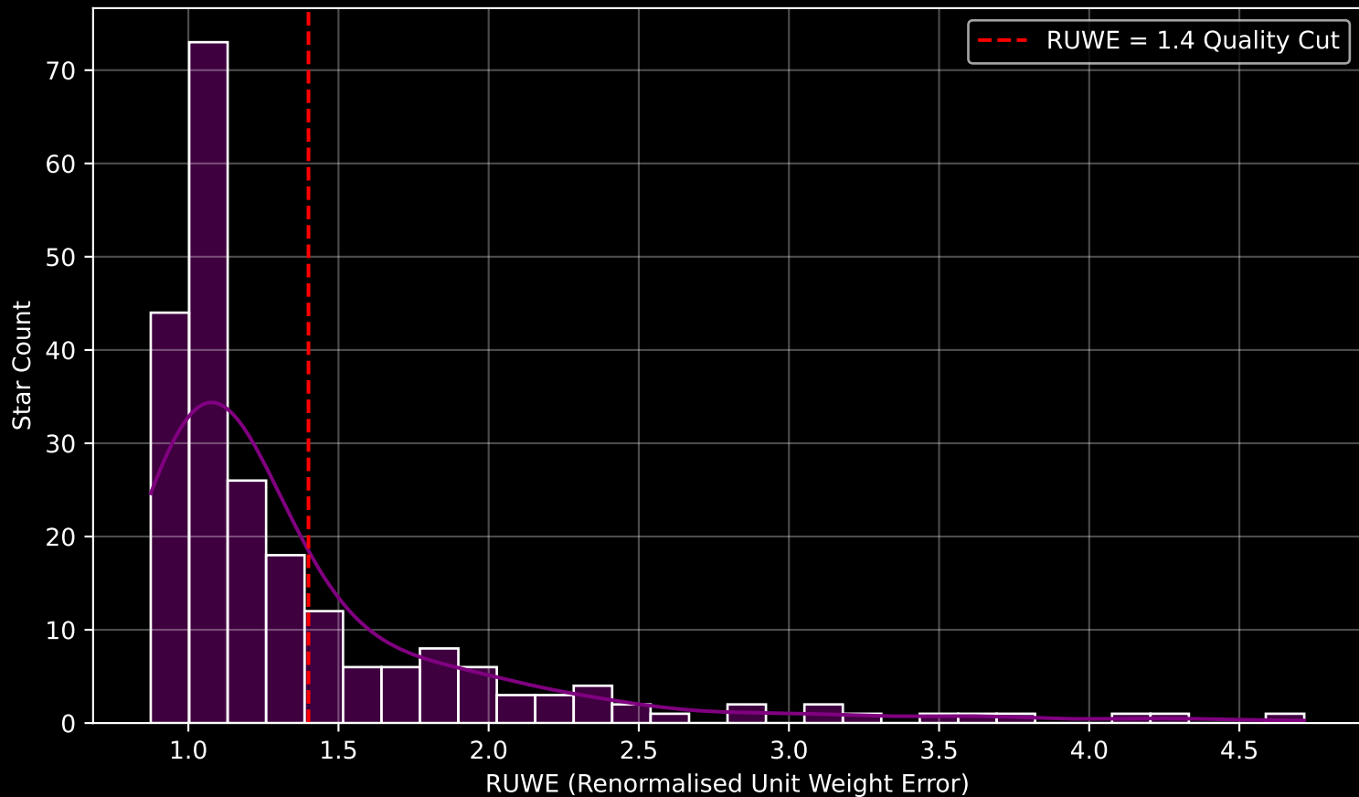
GAPOGEE DR17 Field [040+88_MGA] RUWE Distribution (n= 223)
