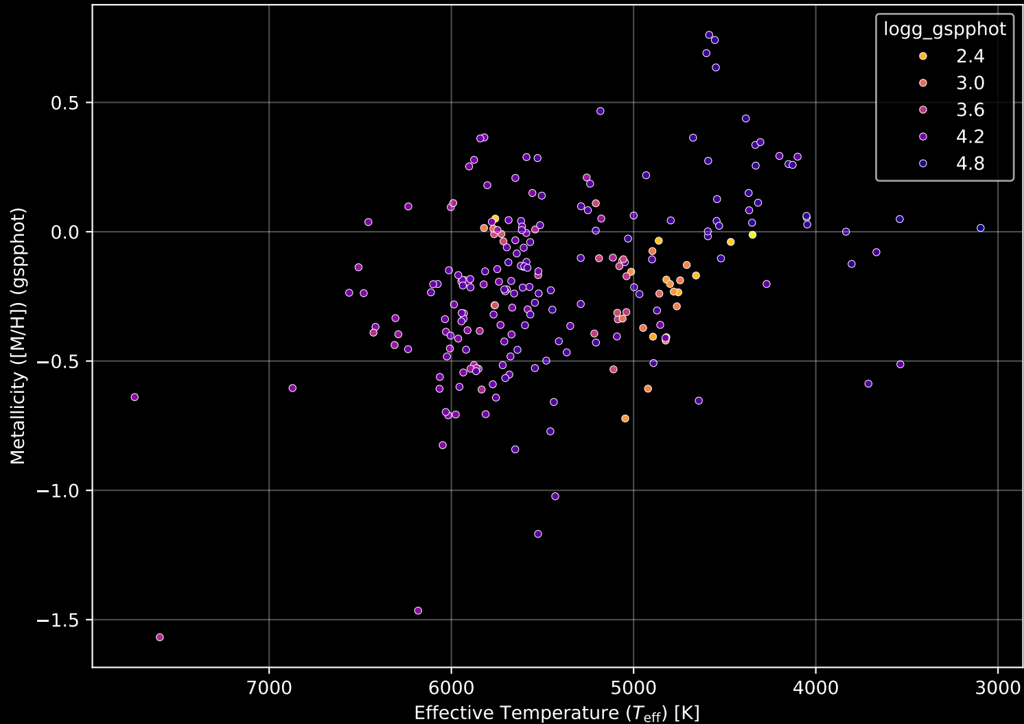
APOGEE DR17 Field: [040+88_MGA] Stellar Population Parameters (n= 231)
