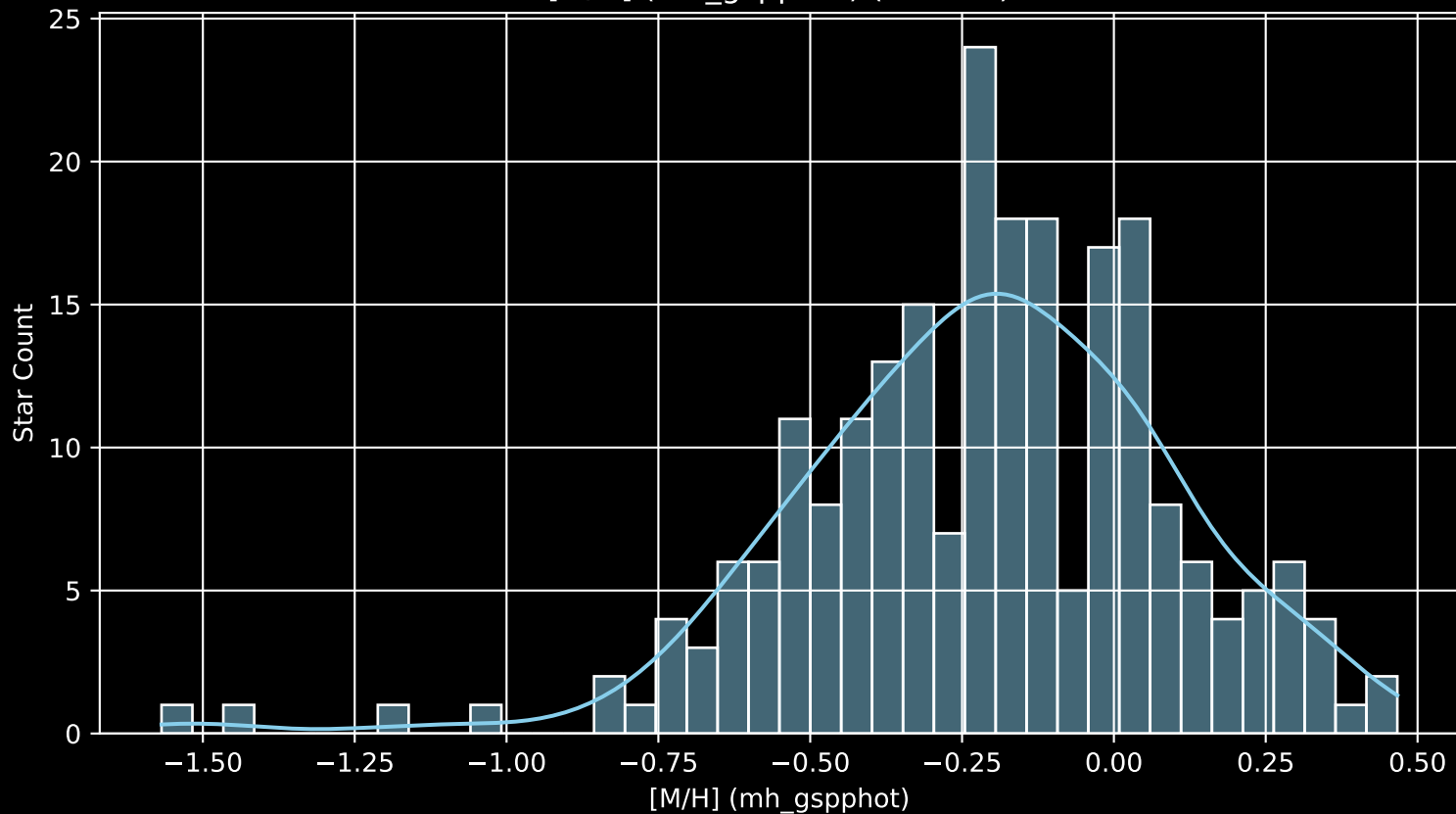
APOGEE DR17 Field: [040+88_MGA [M/H] (mh_gspphot) (n= 227)
