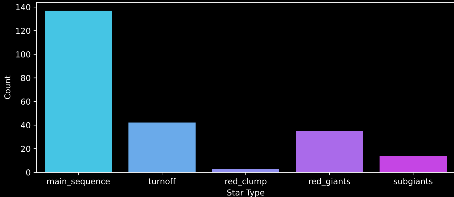
APOGEE DR17 Field: [040+88_MGA] Count plot of Star Type
