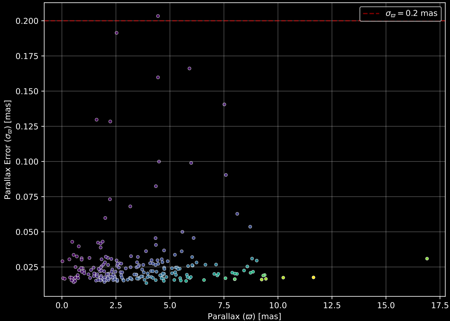
APOGEE DR17 Field: [040+88_MGA] Parallax Quality (n= 231)
